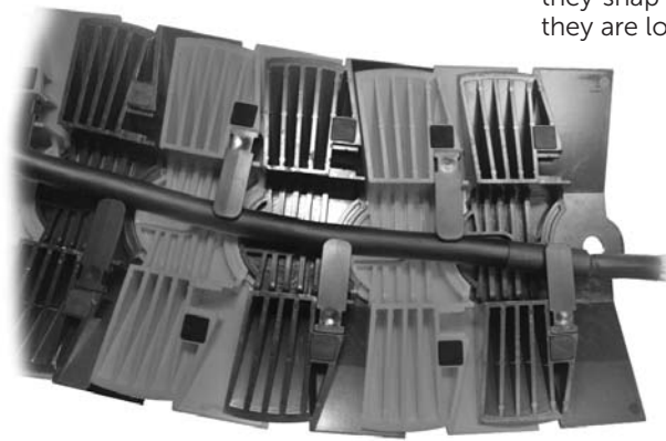
Figure 3: Medium and Large sizes use retainers to secure cables in place
